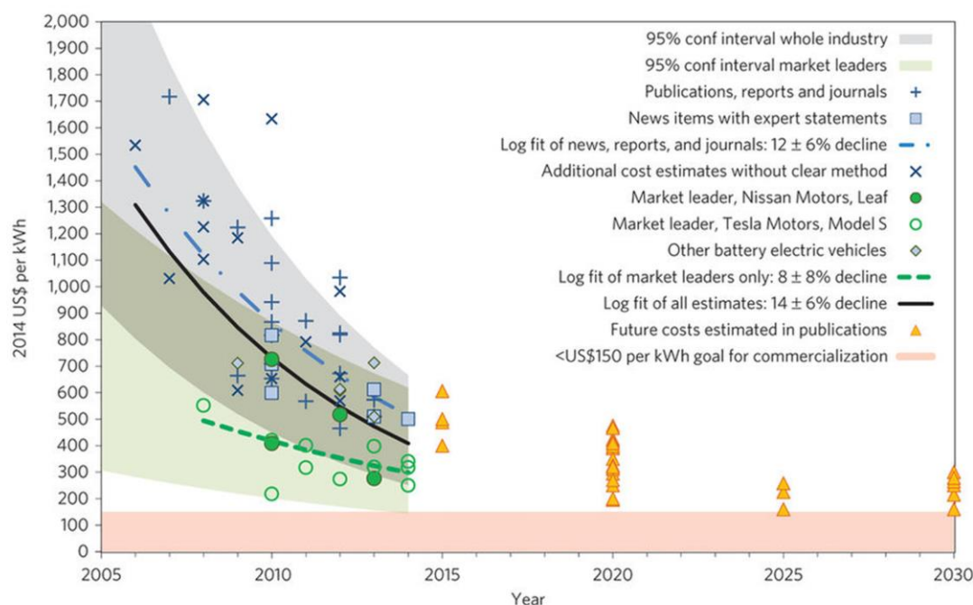
Figure 11: Estimated cost of battery packs in 214 US$/kWh from 2005 to 2014 and forecasts to 2030. Reproduced with permission. [210] Copyright 2015 Springer Nature.
