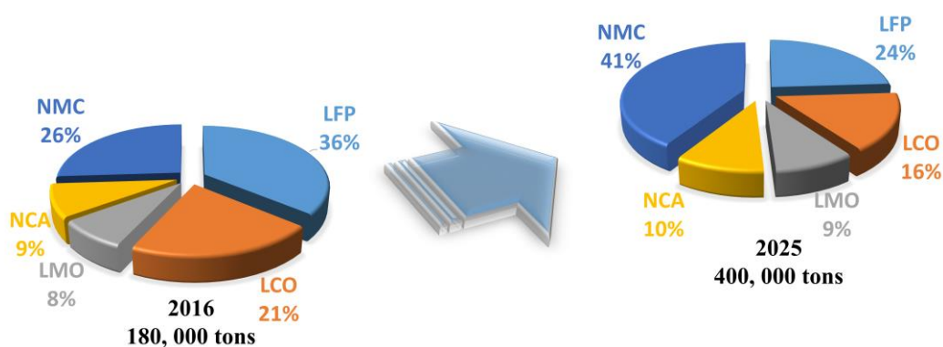
Figure 11: Mass percent of all LIBs market shares of each leading materials in 2016 and forecasted to 2025. [56]
