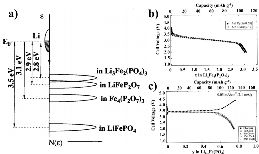
Figure 9: a) The fermi level of \text{Fe}^{3+}/\text{Fe}^{2+} in various structures, charge/discharge voltage profile of b) \text{Li}_x\text{Fe}_4(\text{P}_2\text{O}_7)_3 and c) \text{LiFePO}_4 . [138] Reproduced with permission. [138] Copyright 1997, Electrochemical Society, Inc.
