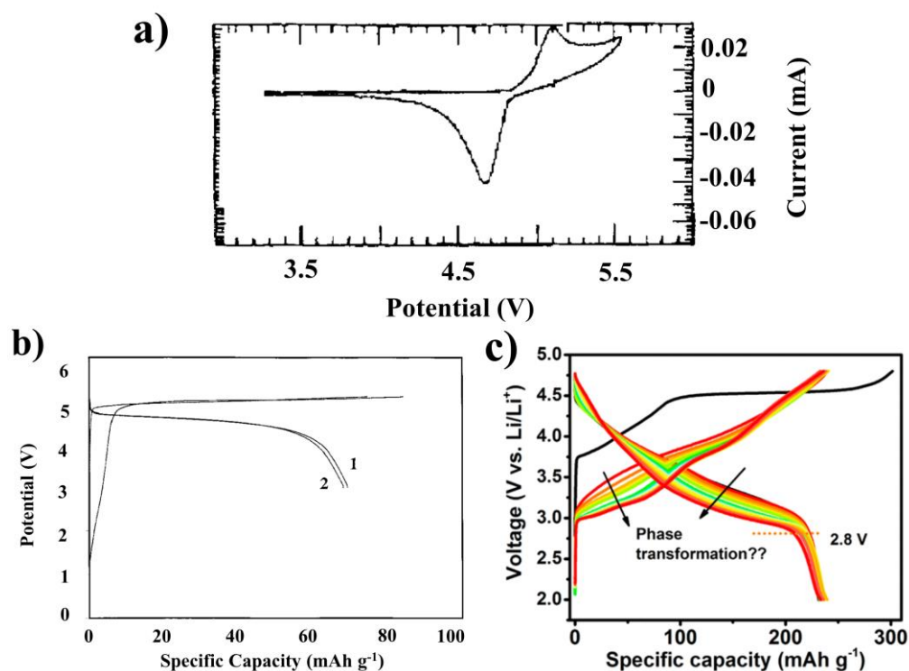
Figure 12: a) Cyclic voltammetry and b) charge discharge profile (1 st and 2 nd cycle) of the 5 V cathode. Reproduced with permission. [220] Copyright 2000 Electrochemical Society, Inc. c) Charge/discharge profiles of LMR, demonstrating its characteristic voltage fade problem. Reproduced with permission. [225] Copyright 2015 American Chemical Society.
