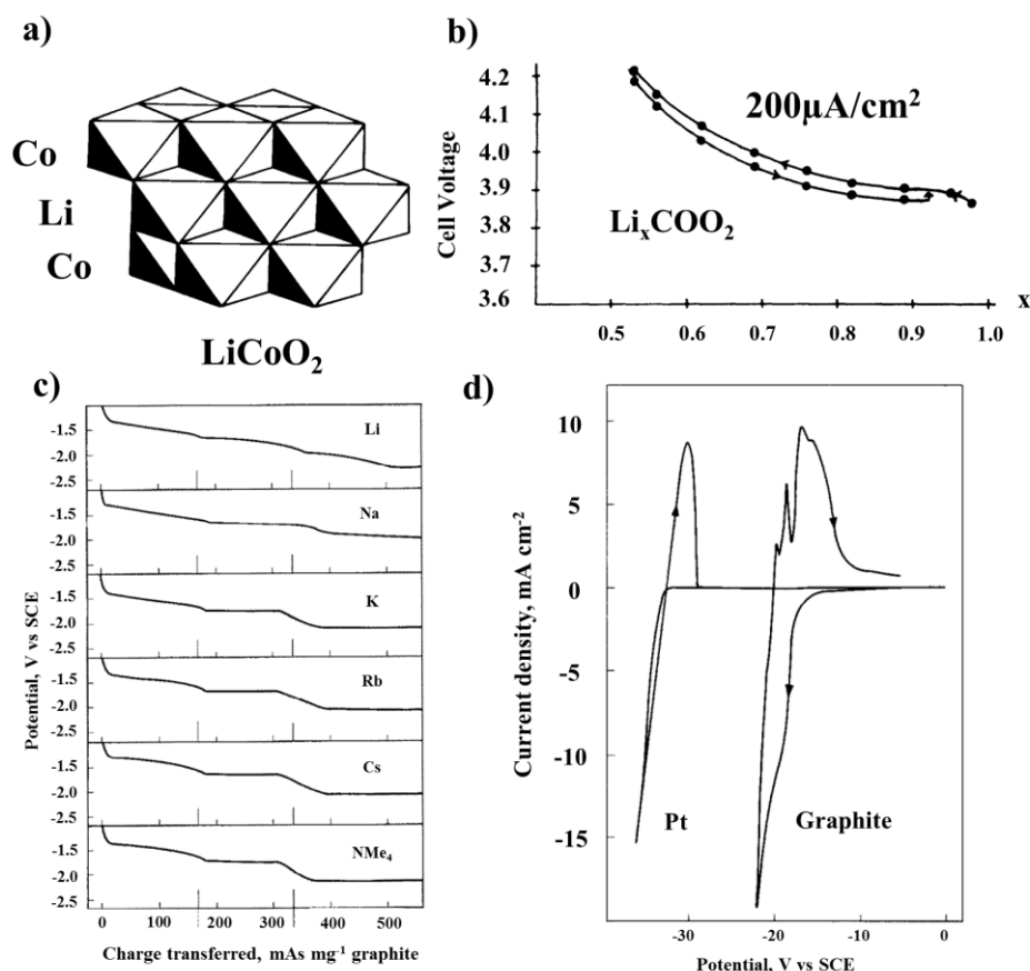
Figure 2: a) The crystal structure of LCO, [18] b) the discharge/charge voltage profile of LCO. Reproduced with permission. [18] Copyright 1980 Elsevier. c) Discharge voltage profile of intercalation of various alkali metals into graphite in \text{LiClO}_4 , \text{NaBF}_6 , \text{KPF}_6 , \text{RbI} , \text{CsI} , \text{NMe}_4\text{Cl/DMSO} and d) cyclic voltammetry of Li-ion intercalation into graphite in 1m \text{LiClO}_4/\text{DMSO} electrolyte. Reproduced with permission. [25] Copyright 1976 Elsevier.
