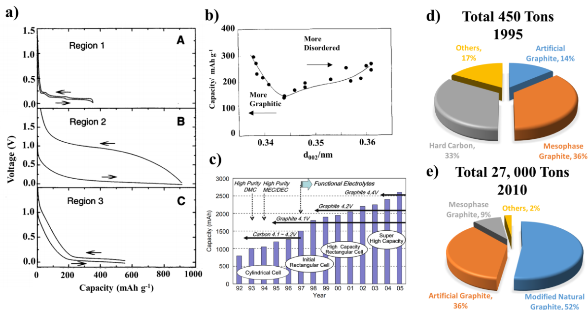
Figure 4: a) Charge/discharge profile for graphitic, hydrogen containing and hard carbon, Reproduced with permission. [43] Copyright 1995 The American Association for the Advancement of Science. b) Relationship between carbon type and capacity. Reproduced with permission. [45] Copyright 1995 Elsevier, c) Absolute capacity in mAh of LIBs from 1992 to 2005 with corresponding technological trends. Reprinted/adapted with permission. [52] Copyright 2009 Springer Nature. d) Approximate market share of various anode materials in d) 1995 and e) 2010, with data estimated from ref. [55]
