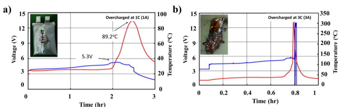
Figure 7: The relationship between temperature and charging voltage during a overcharge test of a LiCoO 2 cell at a) 1C and b) 3C. Reproduced with permission. [117] Copyright 2008, Elsevier.
