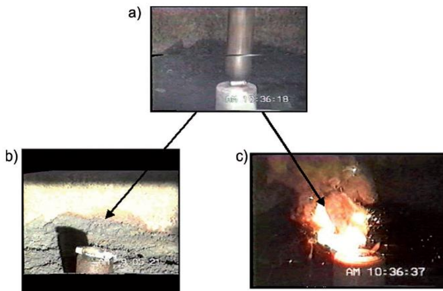
Figure 3: Photos the safety validation tests performed for A. Yoshino: a) image after the cells were impacted with the iron lump, b) A Yoshino's LIB after impact and c) the flaming aftermath of the LMB cell. Reproduced with permission. [37] Copyright 2012 Wiley-VCH.
