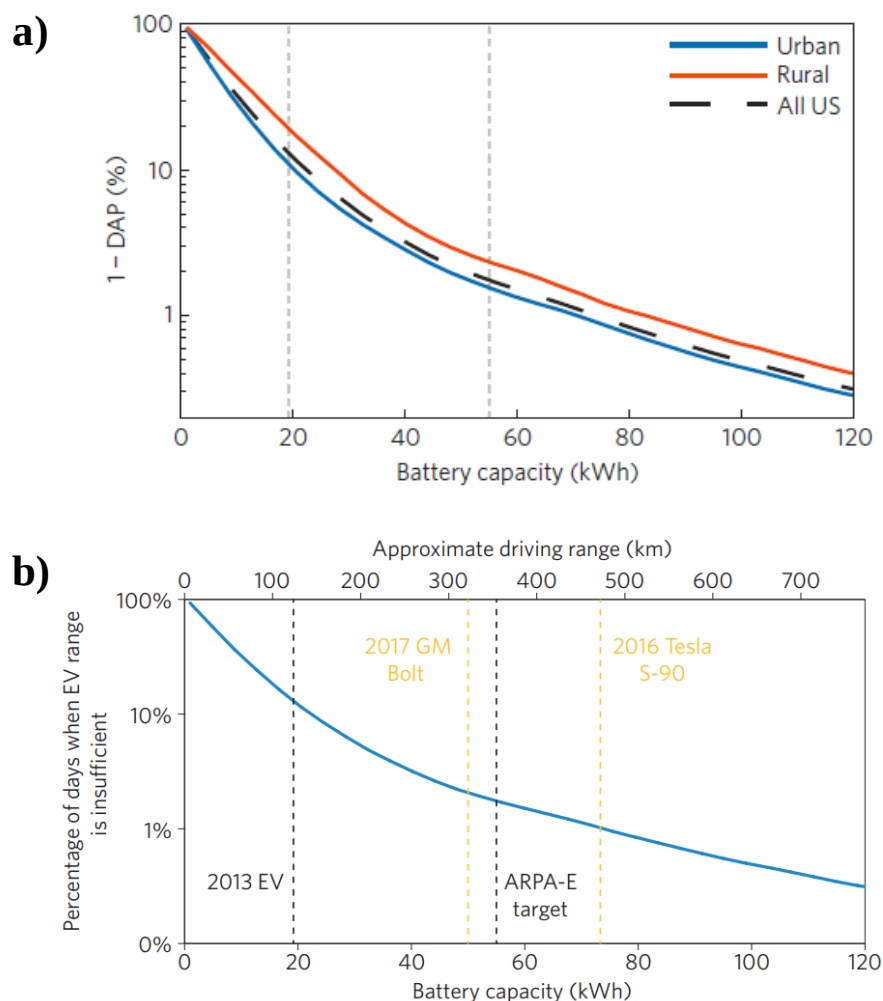
Figure 12: a) The impact of type of driving (urban, rural) in the US on the 1-DAP value. Reproduced with permission. [209] Copyright 2016 Springer Nature. b) The relationship between the % of days when EV range is insufficient (1-DAP) versus the battery capacity and range with the 2013 EV (Nissan Leaf @ 88 Wh kg -1 ) and 2016 Tesla Model S-90 labeled on graph. Reproduced with permission. [212] Copyright 2016 Springer Nature.
