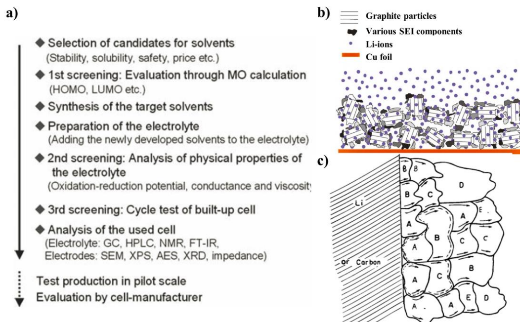
Figure 5: a) New electrolyte identification methodology from Ube Industries Ltd. Reprinted/adapted with permission. [52] Copyright 2009, Springer Nature. b) Schematic of SEI in relation to the anode. Reproduced with permission. [73] Copyright 2010, Elsevier and c) schematic of SEI composition where A=Li 2 O, B=LiF, C=Li 2 CO 3 , D=Polyolefins, and E=Semicarbonates. Reproduced with permission. [74] Copyright 1997, Electrochemical Society, Inc.
